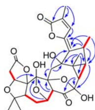
Figure 1. Selected HMBC (from H to C, arrow in blue) and 1 H– 1 H COSY (dash in red) correlations of 1 .
