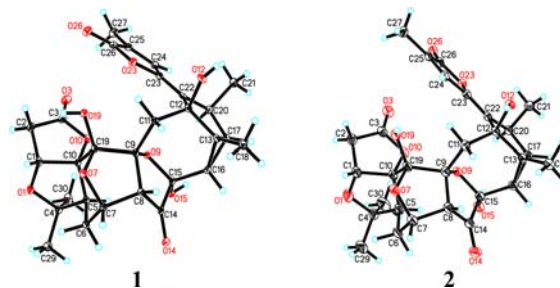
Figure 2. X-ray crystallographic structures of 1 and 2 .
