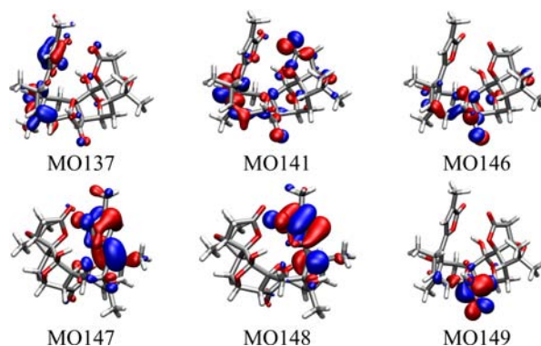
Figure 4. Important MOs in ECD of the optimized conformer 1a at the B3LYP/6-31+G(d,p) level in methanol with PCM model.
