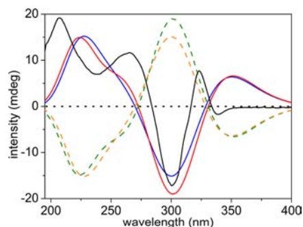
Figure 3. Experimental ECD of 1 (black), calculated ECD of 1 in the gas phase (blue) and in methanol (red), and calculated ECD of ent - 1 in the gas phase (orange) and in methanol (green).
